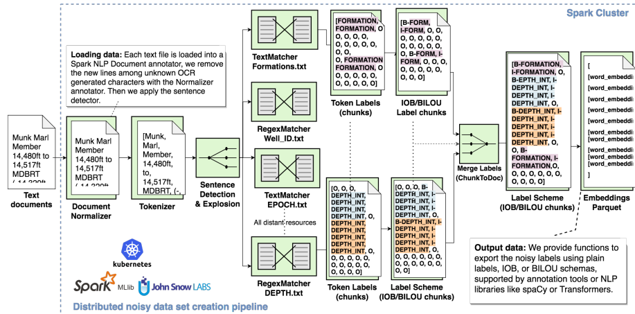
Fig. 3: Spark NLP implementation pipeline
