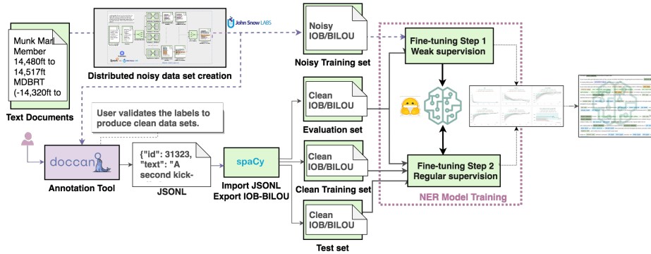
Fig. 2: Implementation pipeline.
